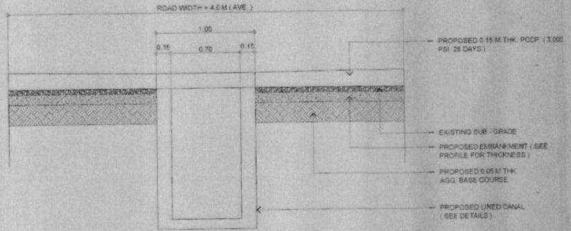
(ZENEDEL HOA) ROAD CROSS SECTION AT ROAD I SCALE: 1:20 M
